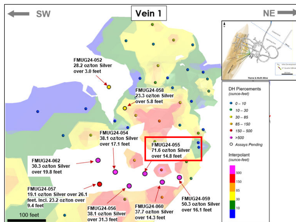
Long section looking West (Azi 302)
